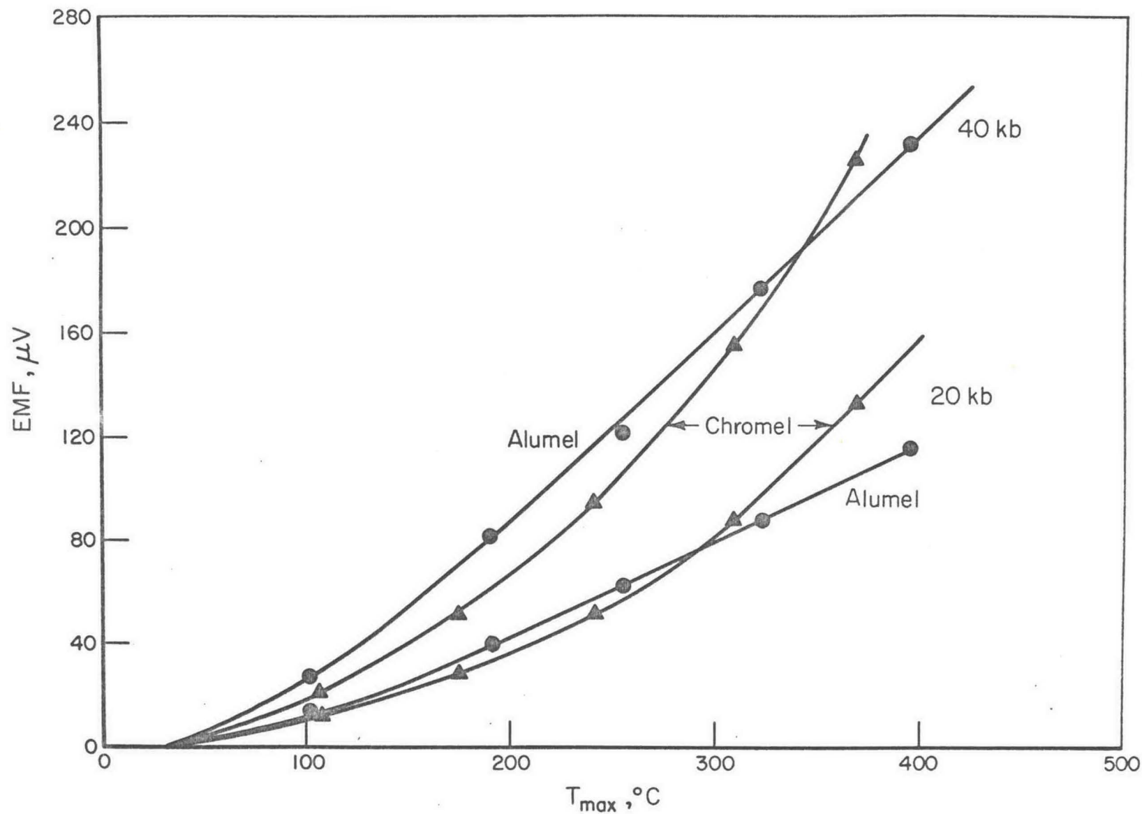
PRESSURE EMF VERSUS TEMPERATURE CHROMEL-ALUMEL Cold + ; hot -
